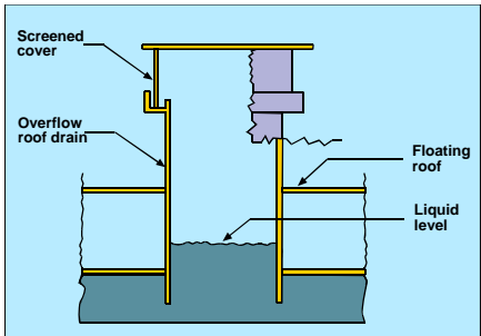
Overflow Drain
