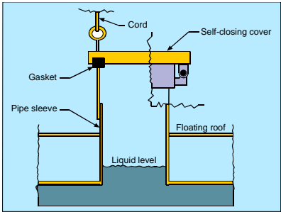
Sample Well
